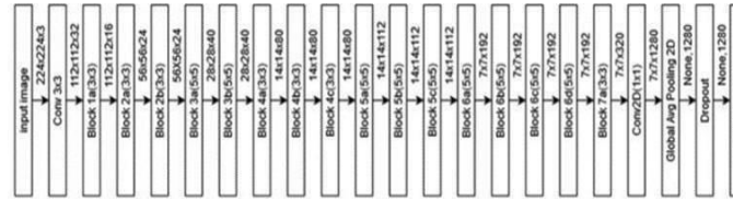
(a) Official EfficientNet B0 Block Diagram.
