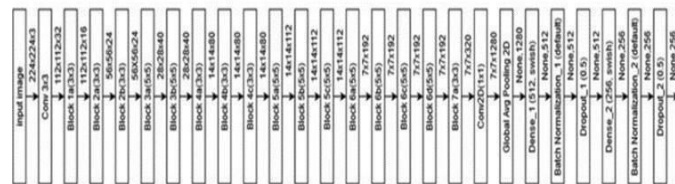
(b) Modified EfficientNet B0 Block Diagram.
